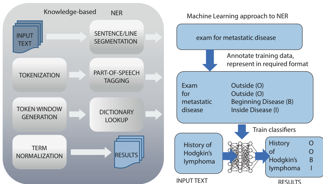
Fig. 8.5 Two approaches to named entity recognition. The approach on the left is a schematic representation of MetaMap – a knowledge-based tool for NER. The right side depicts an abstraction of a machine learning approach to NER. Provided with the following note as input: “Indication: Ca history, exam for metastatic disease, Impression: 1.5 cm nodule in the left midlung zone may contain calcium.” MetaMap will output the following:
